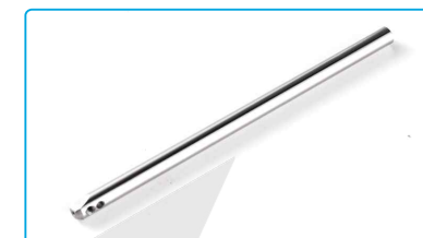
名称: 针杆 Description: Needle Bar 代码/Part NO: 10102002 适配: 普通平车通用 Machine Type: Ordinary lockstitch series
