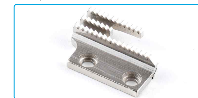
名称: 送布牙 Description: Feed Dog 代码/Part NO: 13514001 适配: JK-6380/6390/H2/H5 Machine Type: JK-6380/6390/H2/H5
