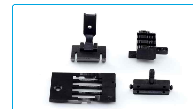
名称: 针位(1) Description: Needle Gauge 1 代码/Part NO: 811004+12915317 适配: JK-58420G/J 58720G/J Machine Type: JK-58420G/J 58720G/J
