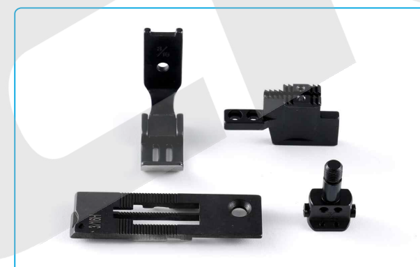
名称: 针位(3/16) Description: Needle Gauge 3/16 代码/Part NO: 810756+12915307 适配: JK-58420G/J 58720G/J Machine Type: JK-58420G 58720G/J
