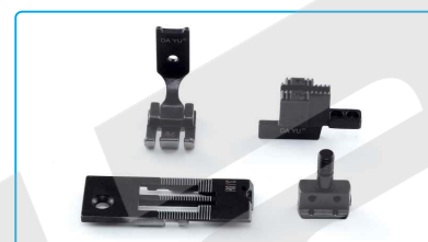
名称: 针位(3/8) Description: Needle Gauge 3/8 代码/Part NO: 810587+12915308 适配: JK-58420G/J 58720G/J Machine Type: JK-58420G/J 58720G/J
