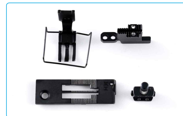
名称: 针位1/4(-3) Description: 58420D Needle Gauge 1/4 (-3) 代码/Part NO: 12915206+11634001+12914301 +1291632500 适配: JK-58420G/J-403 58720G/J-403 Machine Type: JK-58420G/J-403 58720G/J-403
