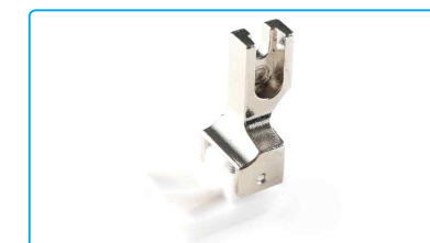
名称: TCR 右高左低1/8塑料压脚 Description: TCR Presser Foot 1/8 代 码/Part NO: 811287 适 配: 平缝机通用 Machine Type: All lockstitch machine series
