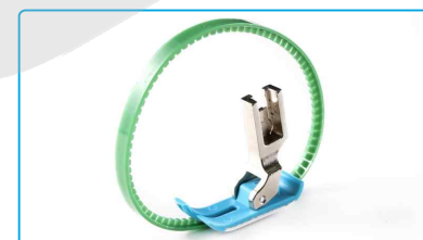
名称: TM-18 塑料左滚轮压脚 Description: TM-18 Presser Foot With Left Roller 代 码/Part NO: 811282 适 配: 平缝机通用 Machine Type: All lockstitch machine series
