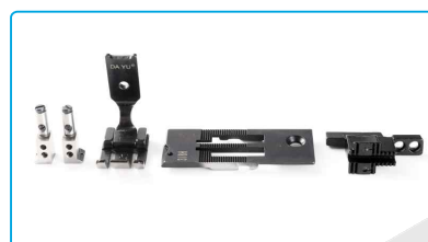
名称: 针位(3/8) Description: Needle Gauge 3/8 代码/Part NO: 810591+12915308 适配: JK-58450G/J 58750G/J Machine Type: JK-58450G/J 58750G/J
