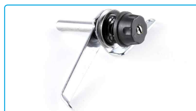
名称: 小夹线器组件 Description: Thread Tension Asm 代码/Part NO: 1381300100 适配: R2/R3/R4E/R4000 Machine Type: R2/R3/R4E/R4000
