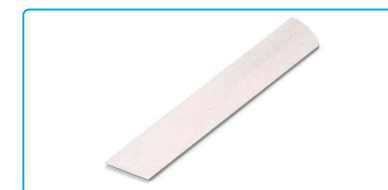
名称: 下刀 Description: Lower Knife 代码/Part NO: 20701053 适配: 包缝E4/C4/C5/C3/797/798T系列所有厚料机型 Machine Type: E4/C4/C5/C3/797/798T overlock series heavy duty models
