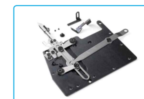
名称: 上切刀组件 Description: Upper Knife Assembly 代码/Part NO: 3101900100 适配: W4-UT/W4E-UT/ W5E-UT/K4-UT/K5-UT Machine Type: W4-UT/W4E-UT/ W5E-UT/K4-UT/K5-UT
