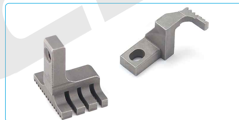
名称: 牙齿组件 Description: Feed Dog Assy 代码/Part NO: 30214008 + 30214009 适配: W4/W4S/K4/K5系列-02BB机型 Machine Type: 02BB type for W4/W4S/K4/K5 series
