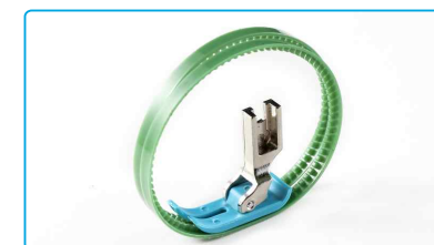
名称: TM-18 塑料双滚轮压脚 Description: TM-18 Presser Foot With Double Roller 代 码/Part NO: 811283 适 配: 平缝机通用 Machine Type: All lockstitch machine series
