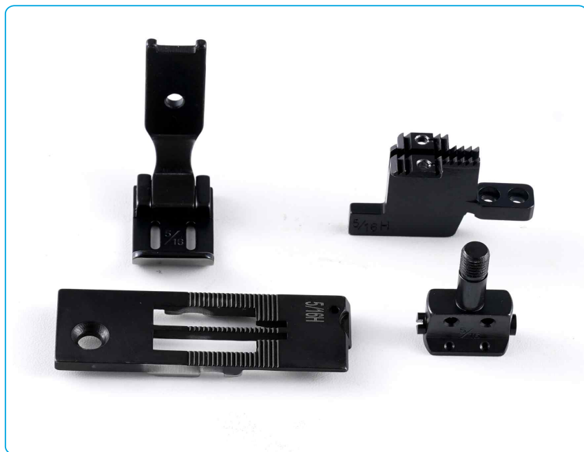
名称: 针位(5/16) Description: Needle Gauge 5/16 代码/Part NO: 804008+12915309 适配: JK-58420G/J 58720G/J Machine Type: JK-58420G/J 58720G/J
