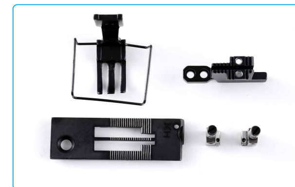
名称: 送布牙1/4(-5) Description: Needle Gauge 1/4 (-5) 代码/Part NO: 11734003+11734002+12914314 +12915206+1291632500 适配: JK-58450G/J-405 58750G/J-405 Machine Type: JK-58450G/J-405 58750G/J-405
