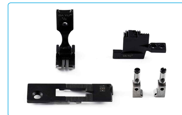
名称: 针位(1/8) Description: Needle Gauge 1/8 代码/Part NO: 810590+12915306 适配: JK-58450G/J 58750G/J Machine Type: JK-58450G/J 58750G/J
