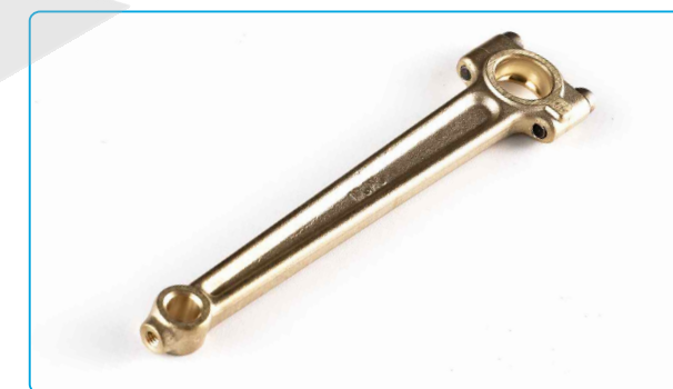
名称: 针杆连杆 Description: Needle Bar Connecting Rod 代码/Part NO: 121205003 适配: 798D/E4/C3 Machine Type: 798D/E4/C3
