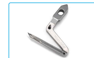
名称: 下弯针 Description: Lower Loper 代码/Part NO: 20717006 适配: 798T/E4/C3/C4/C5 系列(除M03/333机型)外的机型 Machine Type: 798T/E4/C3/C4/C5 series, (Except M03/333 model)
